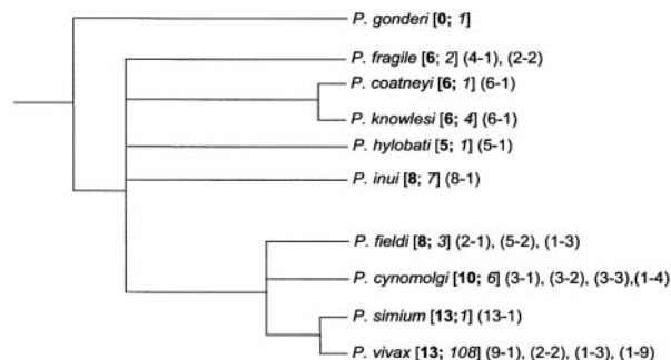
Fig. 1. Consensus phylogenetic tree of 10 Plasmodium species. In brackets, number of shared microsatellite loci in bold; sample size in italics. In parentheses, number of loci–number of alleles per locus.
