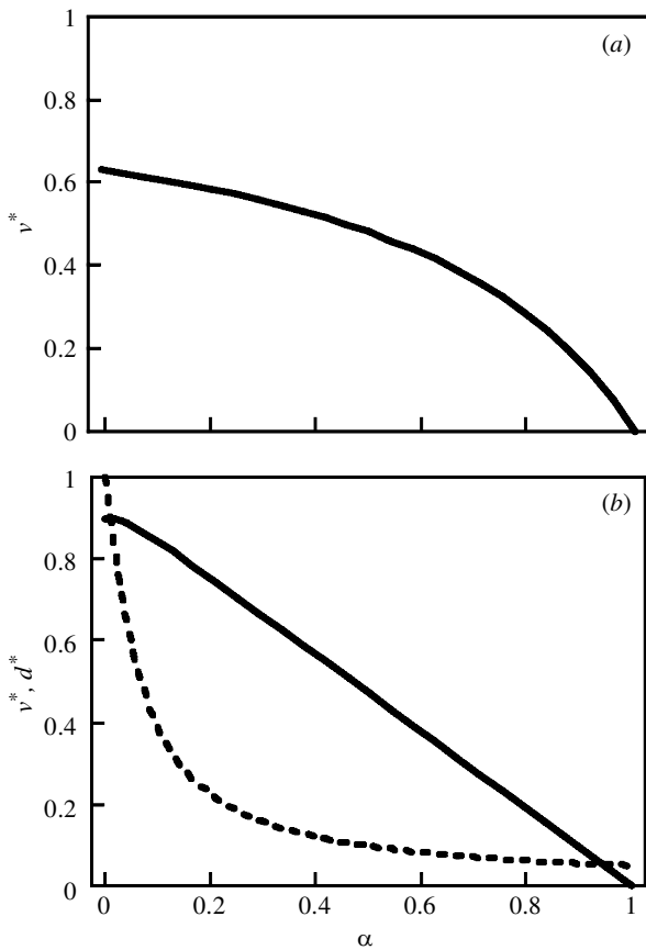
Figure 2. The effect of qualitative resistance ( \alpha ) on the evolution of parasite virulence and dispersal. (a) The evolutionarily stable parasite virulence v^* plotted against qualitative resistance \alpha for N=10 and d=0.1 . (b) Parasite virulence and parasite dispersal coevolve. The evolutionarily stable virulence ( v^* , continuous line) and dispersal ( d^* , dashed line) strategies are plotted against qualitative resistance for N=10 .
