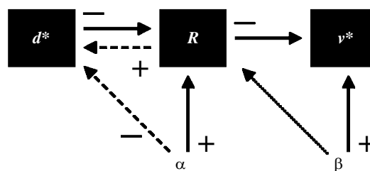
Figure 1. Schematic representation of the effects of qualitative ( \alpha ) and quantitative ( \beta ) forms of resistance on the evolution of parasite virulence ( v^* ) and dispersal ( d^* ) strategies. Qualitative resistance only acts indirectly (via its effect on relatedness R ) on the evolution of virulence while quantitative resistance acts directly. Quantitative resistance could in principle also act indirectly (dotted arrow) but our model does not take into account this effect. The sign by each arrow indicates the main effect of each factor. Dashed arrows represent the case where parasite dispersal is an evolving trait.
