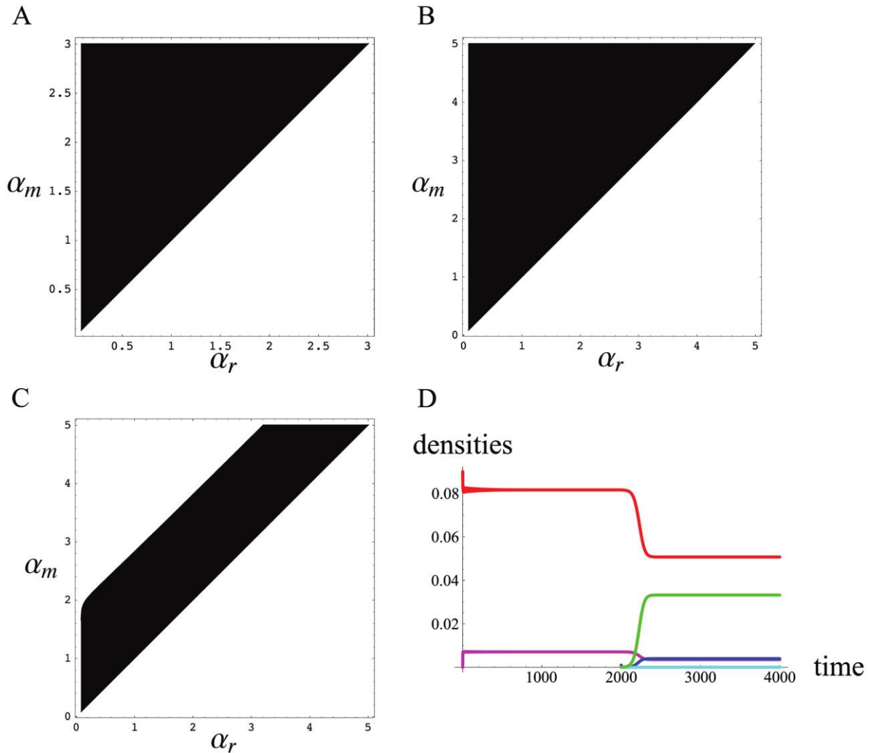
Figure 2: Pairwise invasibility plots with average ( f_1 ; A), high ( f_2 ; B), or low ( f_3 ; C) overall virulence, and coexistence of a virulent and a highly virulent strain in a host population with low overall virulence ( f_3 ; D). A–C show the R_0 of a mutant parasite ( \alpha_m ), depending on the virulence of a resident parasite ( \alpha_r ). In the black areas, the mutant strain disappears ( R_0 < 1 ), while in the white areas, it persists in the host population. Parameter values are \beta = 1 , s = 1 , t = 0.01 , r = 0.1 , and \mu = 0.02 . In D, I start with a virulent strain ( \alpha_1 = 1 ). Hosts infected by the virulent strain ( I_1 ) are in red, and hosts coinfecting by the virulent strain ( D_r ) are in pink. At t = 2,000 , I introduce a rare, highly virulent strain ( \alpha_2 = 4 ). Hosts infected by only the mutant strain ( I_m ) are in blue, while hosts coinfecting by the mutant strain ( D_{mm} ) are in cyan. Hosts coinfecting by two different strains are in green.
