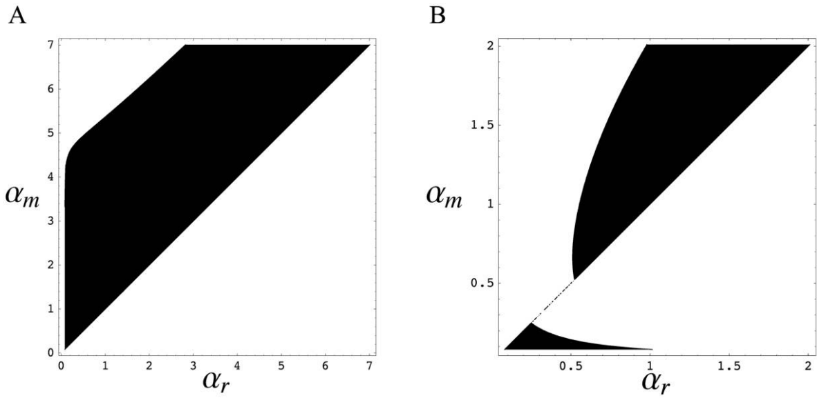
Figure B2: R_0 of a mutant parasite ( \alpha_m ) in a population infected by a resident parasite ( \alpha_r ) in a case without (A) or with (B) a transmission-virulence trade-off. In A, parameter values are identical to those in figure 2, and in B, they are identical to those in figure 3.
