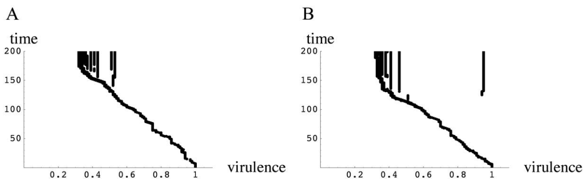
Figure B3: Evolutionary dynamics of the trait with small mutations (A) and with occasional large mutations (B). Parameter values are a = 1 , s = 1 , t = 0.01 , r = 0.1 , and \mu = 0.02 .
