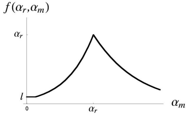
Figure B1: Overall virulence in a coinfecting host. The first strain has a virulence \alpha_r , and the second strain has a virulence \alpha_m . The function is centered in \alpha_m = \alpha_r , but it is not symmetric. Parameter values are s = 1 .
