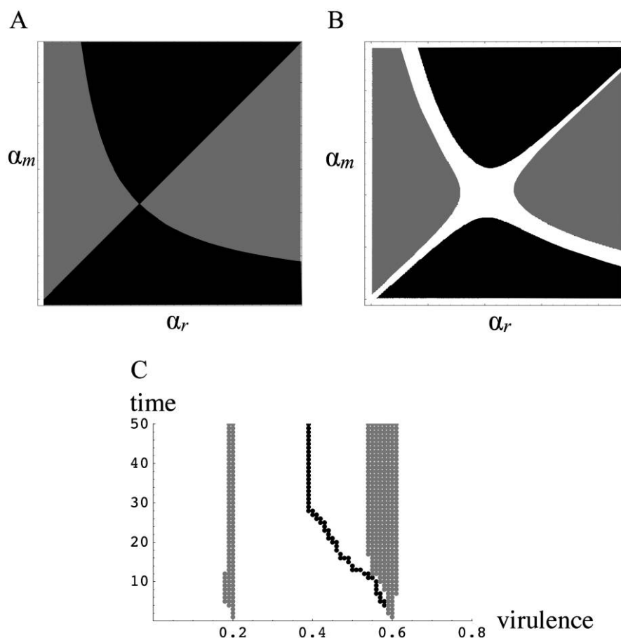
Figure C1: Pairwise invasibility plots with (A) and without (B) hosts coinfecting by the same strain. In the black regions, the mutant can invade and replace the resident; in gray areas, it is the opposite; and in white areas, both the mutant and the resident can invade each other (which implies coexistence). The evolutionary dynamics are shown in C; case A is in black, and case B is in gray. Parameter values are r = 0.25 and \mu = 0.2 .
