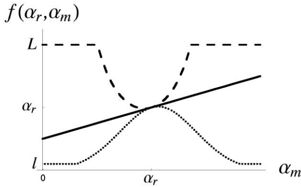
Figure 1: Overall virulence in a coinfecting host. Overall virulence can be an average function ( f_1 ; solid line), an increasing function ( f_2 ; dashed line), or a decreasing function ( f_3 ; dotted line). The first strain that arrives in the host has a virulence \alpha_r , and the second strain has a virulence \alpha_m . The minimum and maximum overall virulence values are denoted l and L , respectively. In this figure, s = 1 .
