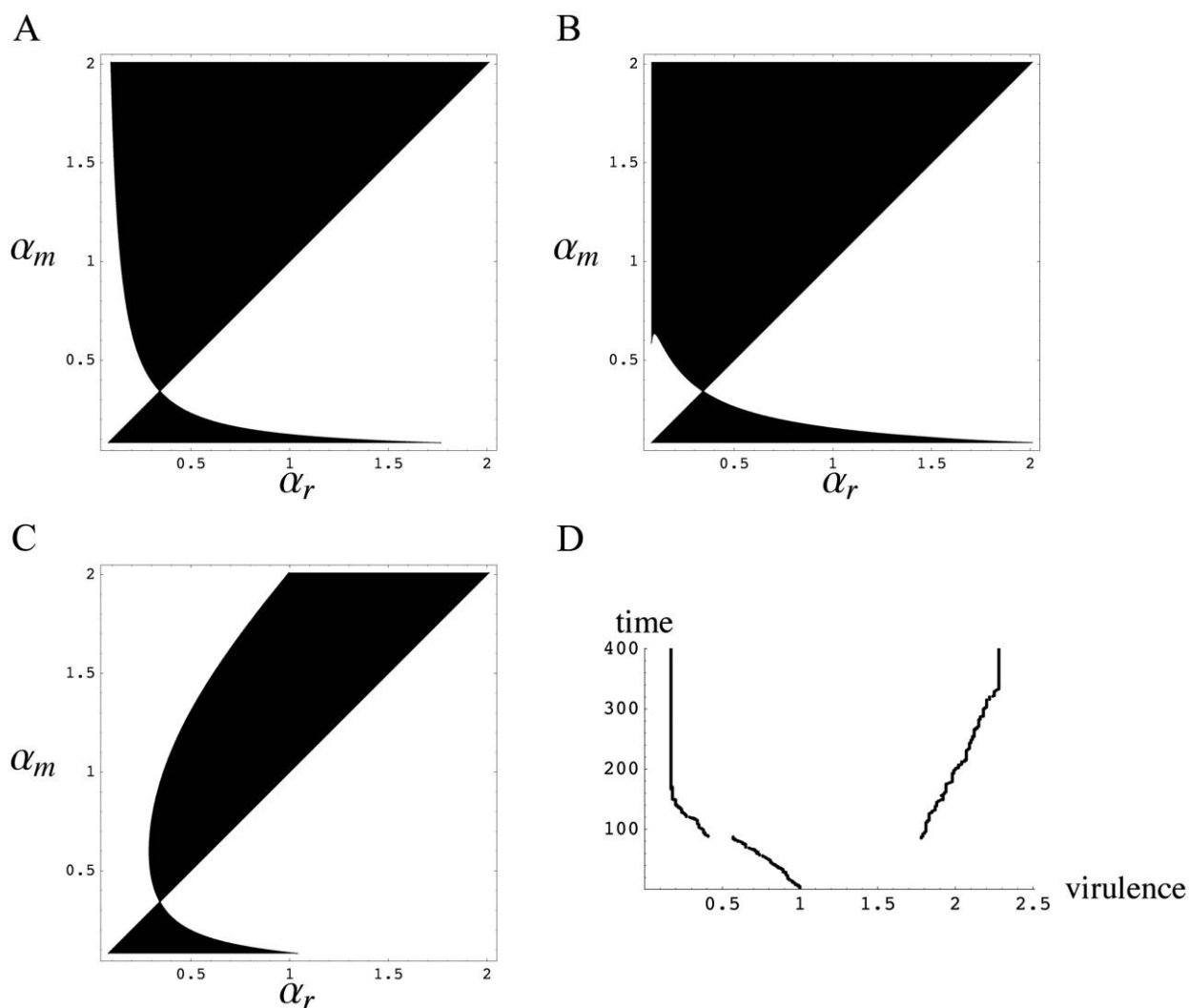
Figure 3: Pairwise invasibility plots with a transmission-virulence trade-off for average (A), high (B), and low (C) overall virulence, and evolutionary dynamics of the virulence trait for low overall virulence (D). Parameter values are a = 1 , s = 1 , t = 0.01 , r = 0.1 , and \mu = 0.02 . In D, mutation rate is 10^{-5} , and the mutation step is 0.01 for small mutations. For further details, see figure 2.
