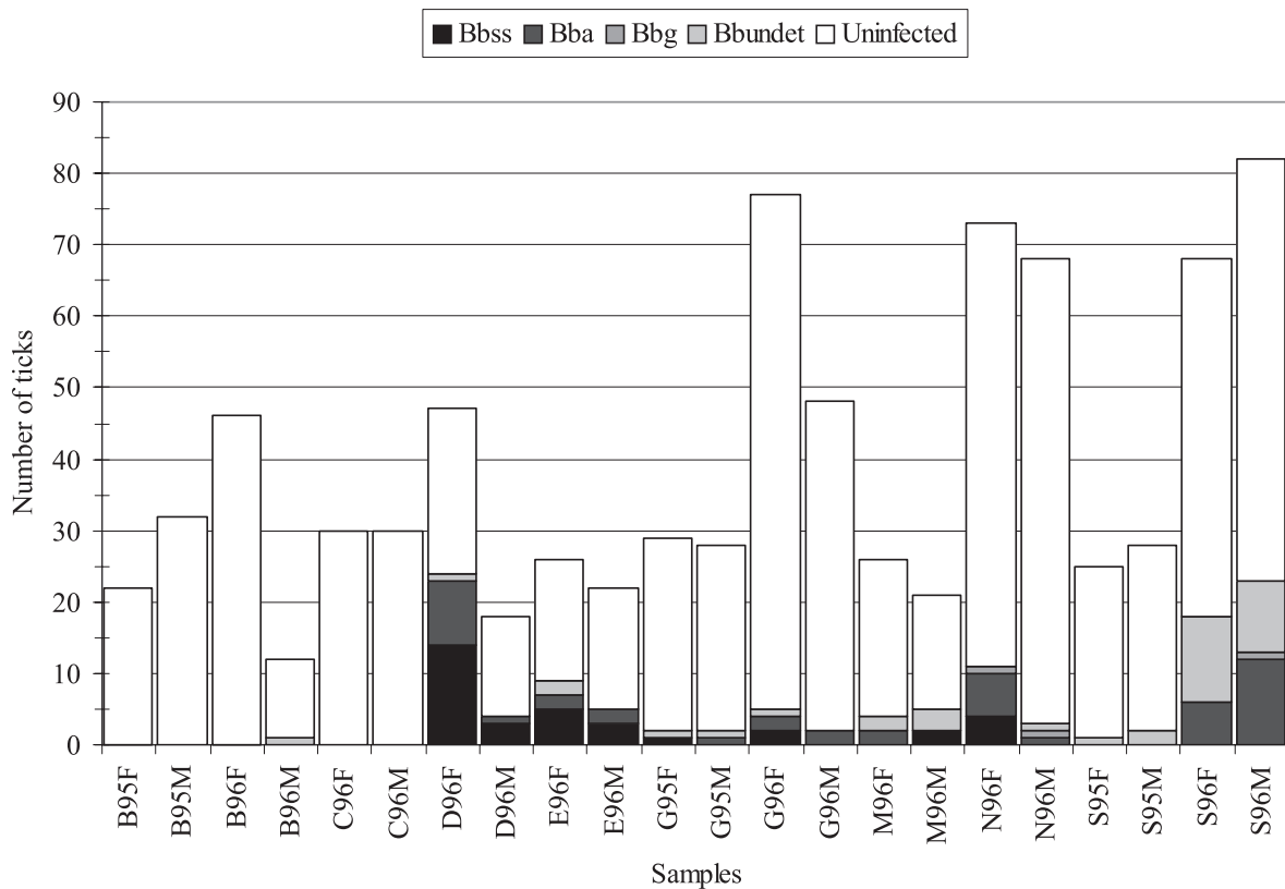
Fig. 1. Number of I. ricinus infected by the different B. burgdorferi genospecies in the different female (F) and male (M) tick samples in years 1995 (95) and 1996 (96). B = Bern, C = Monte Ceneri, D = Dorenaz, E = Eclepens, G = Gorges du Trient, M = Montmollin, N = Neuchâtel, S = Staadswald; see [4] for sample locations.
