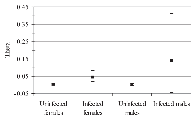
Fig. 2. The different values of \theta ( F_{st} estimator) obtained for uninfected and infected female and male ticks. The 95% confidence intervals were obtained after bootstrapping over loci.
