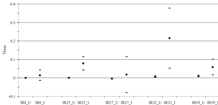
Fig. 3. The different values of \theta ( F_{st} estimator) obtained for uninfected (U) and infected (I) ticks for each of the five microsatellite loci (IR8, IR25, IR27, IR32 and IR39). The 95% confidence intervals were obtained after jack-knifing over populations.
