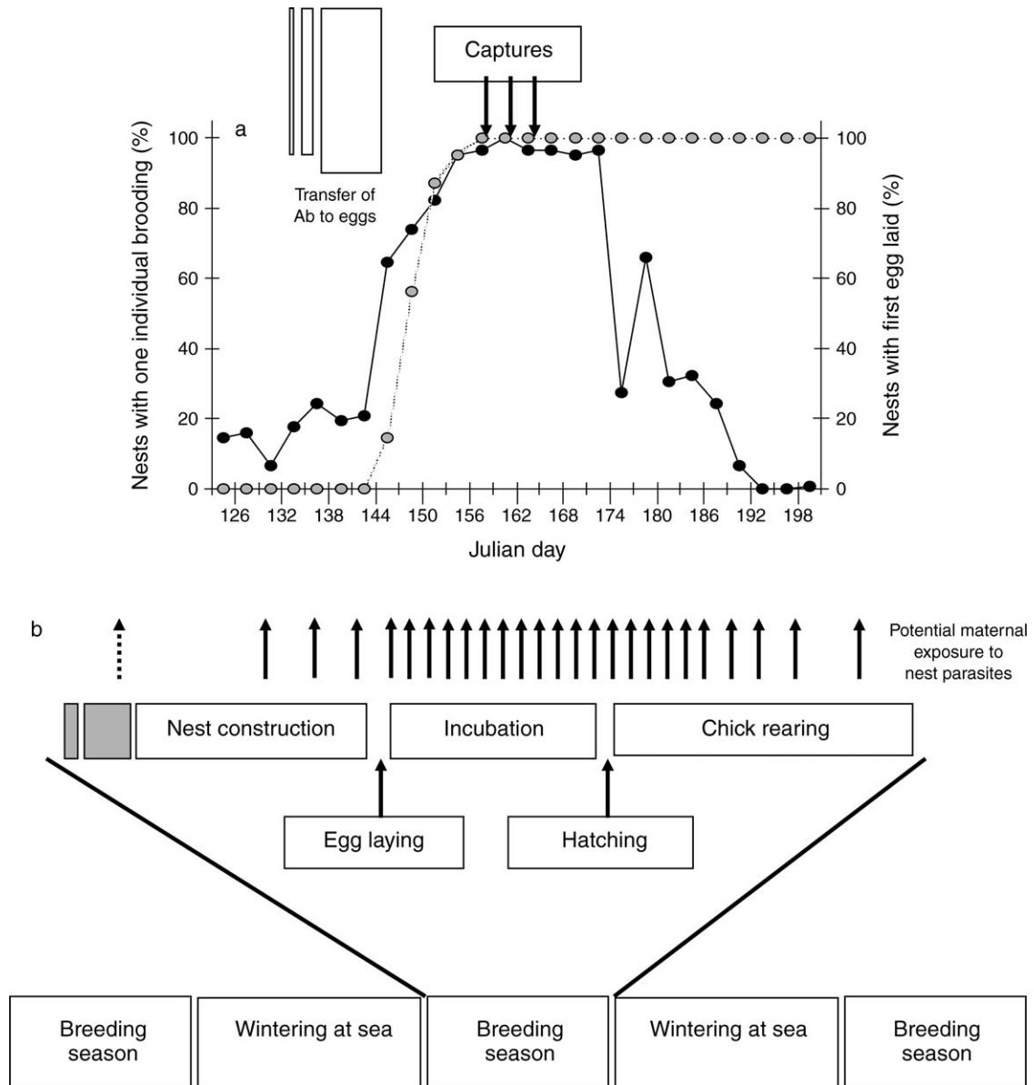
FIG 1. Time frame of the interaction between the parasite and the host immune system for the Black-legged Kittiwake Rissa tridactyla . (a) Black circles represent the percentage of nests with a brooding individual among nests where at least one egg will be laid during the season, and gray circles represent the percentage of nests with a first egg laid (data are from 2005, but the same pattern is observed every year). Julian day 1 is 1 January. Here, brooding means sitting on a nest. Adult birds were captured during incubation. (b) Because maternal exposure to nest parasites (general pattern indicated by solid arrows) is probably negligible before egg laying, the transfer of maternal antibodies (Ab) to the eggs occurs before peak exposure to nest parasites. The immunological memory targeted against nest parasites and acquired during incubation and chick rearing in one breeding season may therefore be key for the transfer of adequate Ab to the chicks in the subsequent season. At the left, the gray boxes and dotted arrow indicate potential, but rare, exposure to parasites for birds that begin nest construction ahead of the main period.
